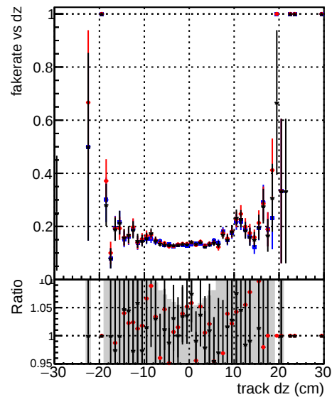
DOM-pixelCPE+template step2 ttbar-phase1-newgeom DOM-pixelCPE+templateCutChiSquareNew7_step2 ttba
