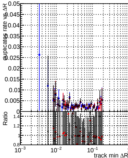
—■— DQM_original_step2_ttbar-phase1-newgeom —●— DQM_pixelCPETemplate_step2_ttbar-phase1-newgeom —▲— DQM_pixelCPETemplateCutChiSquareNew7_step2_ttbar-phase1-newgeom
