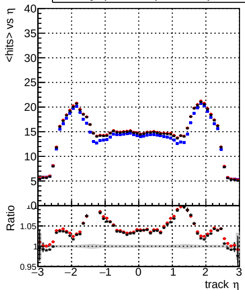
mean hits vs \eta — DQM_original_step2_ttbar-phase1-newgeom — DQM_pixelCPETemplate_step2_ttbar-phase1-newgeom — DQM_pixelCPETemplateCutChiSquareNew7_step2_ttbar-phase1-newgeom
