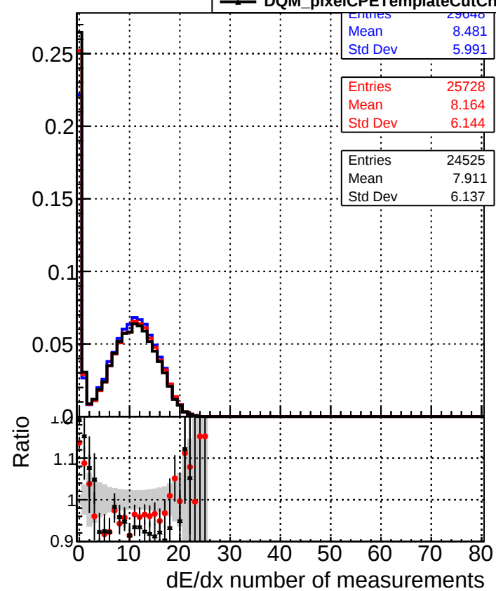
— DQM_original_step2_ttbar-phase1-newgeom — DQM_pixelICPETemplate_step2_ttbar-phase1-newgeom — DQM_pixelICPETemplateCutChiSquareNew7_step2_ttbar-phase1-newgeom
