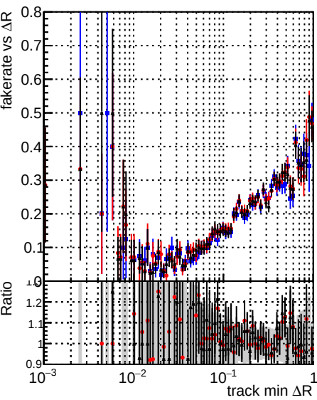
Fake rate vs \Delta R (track, jet) DQM original step2 ttbar-phase1-newgeom DQM pixelCPETemplate step2 ttbar-phase1-newgeom DQM pixelCPETemplateCutChiSquareNew7_step2_ttbar-phase1-newgeom
