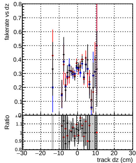
Fake rate vs dz Legend: DOM original_step2_tbar-phase1-newgeom DOM pixelCPE-template-step2_tbar-phase1-newgeom DOM pixelCPE-template-cutchisquare-new/step2_tbar-phase1-newgeom
