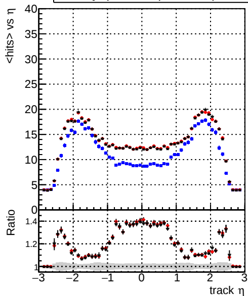
mean hits vs \eta Legend: DQM_original_step2_ttbar-phase1-newgeom (blue line) DQM_pixelCPETemplate_step2_ttbar-phase1-newgeom (red line) DQM_pixelCPETemplateCutChiSquareNew7_step2_ttbar-phase1-newgeom (black line)
