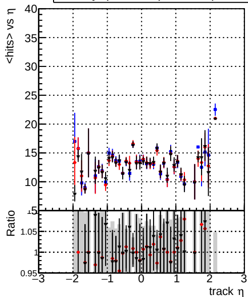
mean hit — DQM_original_step2_ttbar-phase1-newgeom — DQM_pixelCPETemplate_step2_ttbar-phase1-newgeom — DQM_pixelCPETemplateCutChiSquareNew7_step2_ttbar-phase1-newgeom
