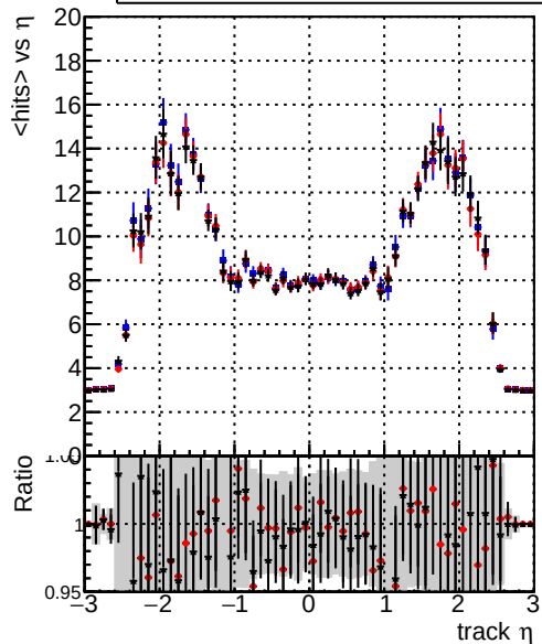
mean hits vs \eta — DQM_original_step2_ttbar-phase1-newgeom — DQM_pixelCPETemplate_step2_ttbar-phase1-newgeom — DQM_pixelCPETemplateCutChiSquareNew7_step2_ttbar-phase1-newgeom
