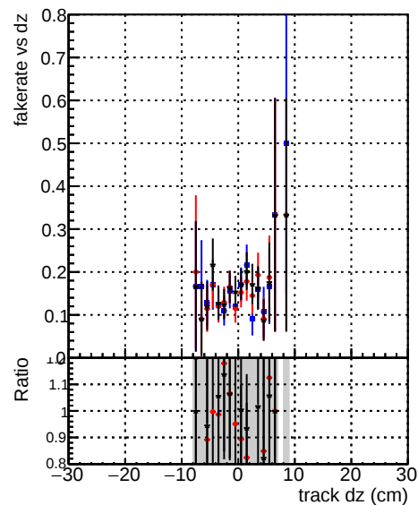
Fake rate vs dz Legend: DOM original_step2_ttbarenewgeom DOM pixelCPEtemplate_step2_ttbarenewgeom DOM pixelCPEtemplatecutchisquarenew_step2_ttbarenewgeom
