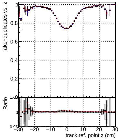
—●— DQM_original_step2_ttbbar-phase1-newgeom —●— DQM_pixelCPETemplate_step2_ttbbar-phase1-newgeom —●— DQM_pixelCPETemplateCutChiSquareNew7_step2_ttbbar-phase1-newgeom
