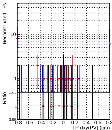
2_ttbar-phase1-newgeom
