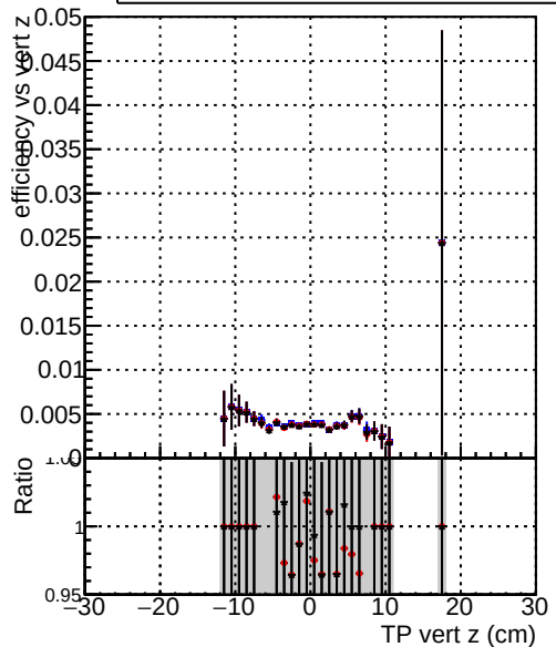
— DQM_original_step2_ttbbar-phase1-newgeom — DQM_pixelCPETemplate_step2_ttbbar-phase1-newgeom — DQM_pixelCPETemplateCutChiSquareNew7_step2_ttbbar-phase1-newgeom
