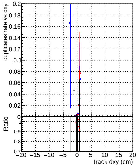
ttbar-phase1-newgeom squareNew7 step2 ttbar-ph
