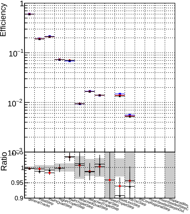
DQM_original_step2_ttbar-phase1-newgeom DQM_pixelICPETemplate_step2_ttbar-phase1-newgeom DQM_pixelICPETemplateCutChiSquareNew6_step2_ttbar-phase1-newgeom
