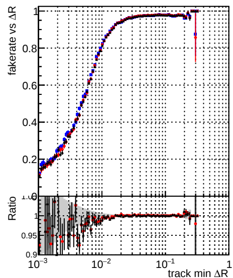
Legend: - DQM_original_step2_ttbar-phase1-newgeom (blue squares) - DQM_pixelCPETemplateCut2_ttbar-phase1-newgeom (red circles) - DQM_pixelCPETemplateCutChiSquareNew6_step2_ttbar-phase1-newgeom (black crosses)
