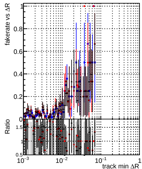
—●— DQM_original_step2_ttbar-phase1-newgeom —●— DQM_pixelCPETemplateCut2_ttbar-phase1-newgeom —●— DQM_pixelCPETemplateCutChiSquareNew6_step2_ttbar-phase1-newgeom
