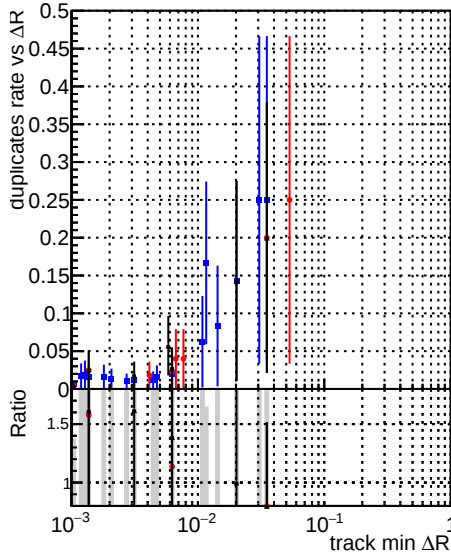
—●— DQM_original_step2_ttbar-phase1-newgeom —●— DQM_pixelCPETemplateCut2_ttbar-phase1-newgeom —●— DQM_pixelCPETemplateCutChiSquareNew6_step2_ttbar-phase1-newgeom
