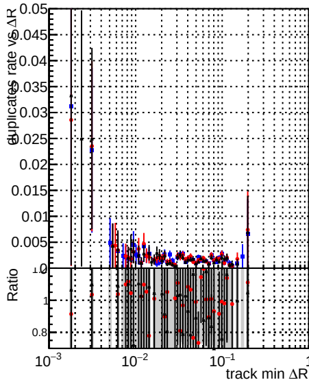
—●— DQM_original_step2_ttbar-phase1-newgeom —●— DQM_pixelCPETemplate_step2_ttbar-phase1-newgeom —●— DQM_pixelCPETemplateCutChiSquareNew6_step2_ttbar-phase1-newgeom
