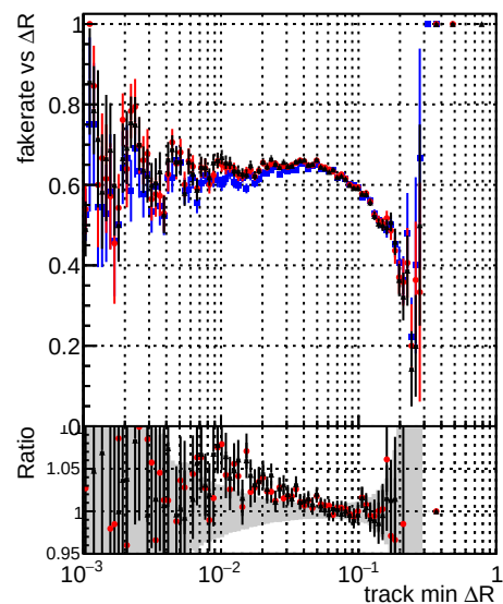
—●— DQM_original_step2_ttbar-phase1-newgeom —●— DQM_pixelCPETemplate_step2_ttbar-phase1-newgeom —●— DQM_pixelCPETemplateCutChiSquareNew6_step2_ttbar-phase1-newgeom
