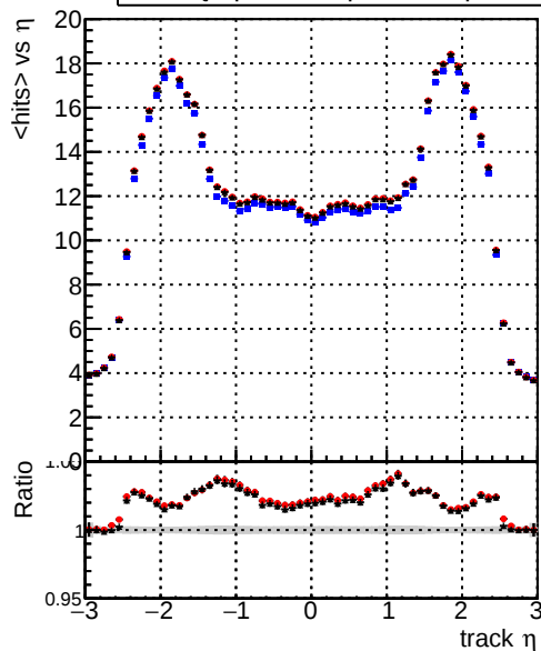
mean hits — DQM_original_step2_ttbar-phase1-newgeom — DQM_pixelCPETemplate_step2_ttbar-phase1-newgeom — DQM_pixelCPETemplateCutChiSquareNew6_step2_ttbar-phase1-newgeom
