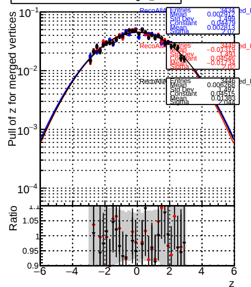
RecoAllAssoc2GenMatchedMerged_PullIZ
