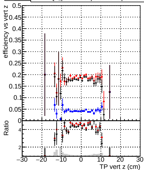
Efficiency vs vert z — DQM_original_step2_ttbbar-phase1-newgeom — DQM_pixelCPETemplate_step2_ttbbar-phase1-newgeom — DQM_pixelCPETemplateCutChiSquareNew6_step2_ttbbar-phase1-newgeom
