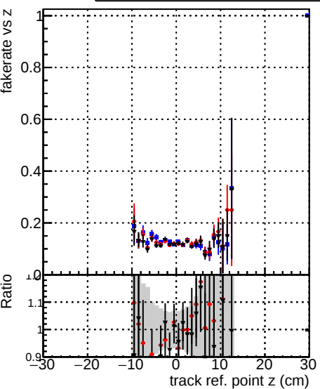
Fake rate vs verpos — DQM_original_step2_ttbar-phase1-newgeom — DQM_pixelCPETemplate_step2_ttbar-phase1-newgeom — DQM_pixelCPETemplateCutChiSquareNew6_step2_ttbar-phase1-newgeom
