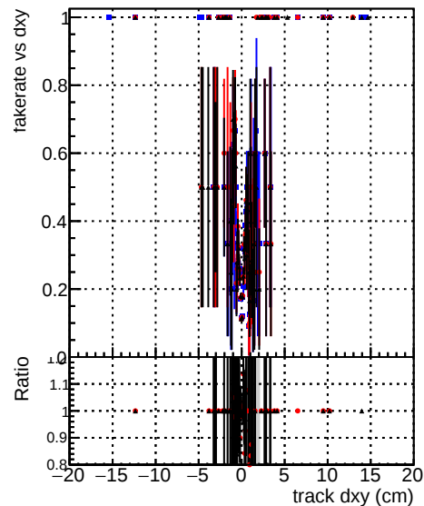
DOM original step2 tbar-phase1-newgeom DOM pixel CPE template step2 tbar-phase1-newgeom DOM pixel CPE template cutchisquareNew step2 tbar-phase1-newgeom
