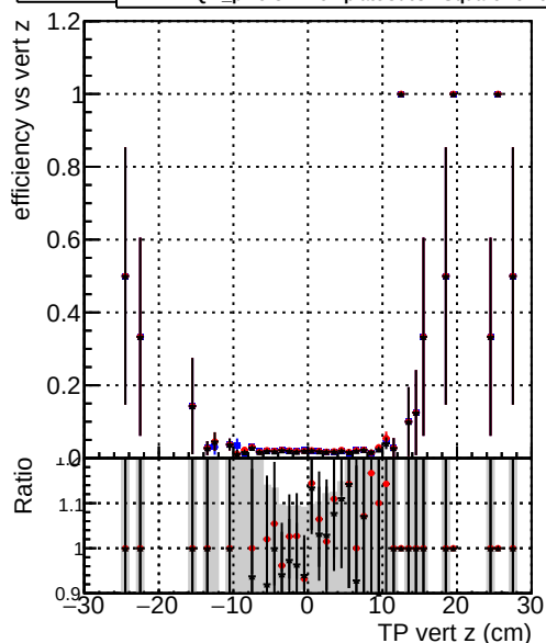
Efficiency vs vert z —●— DQM_original_step2_ttbare-phase1-newgeom —●— DQM_pixelCPETemplate_step2_ttbare-phase1-newgeom —●— DQM_pixelCPETemplateCutChiSquareNew6_step2_ttbare-phase1-newgeom
