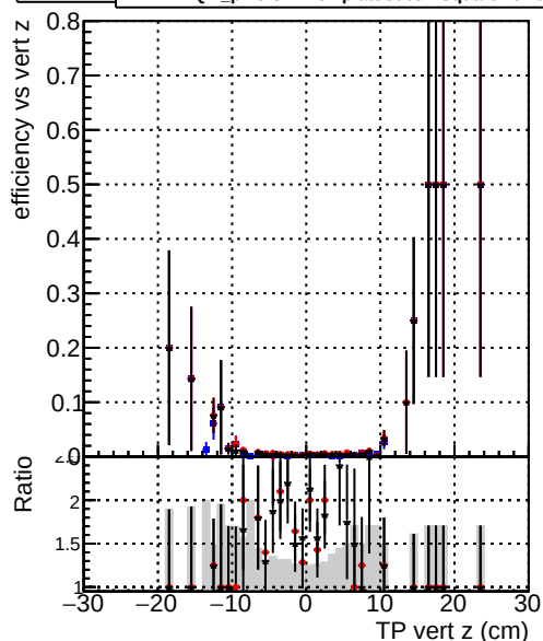
Efficiency vs. TP vert z (cm) —•— DQM_original_step2_ttbbar-phase1-newgeom —•— DQM_pixelCPETemplate_step2_ttbbar-phase1-newgeom —•— DQM_pixelCPETemplateCutChiSquareNew6_step2_ttbbar-phase1-newgeom
