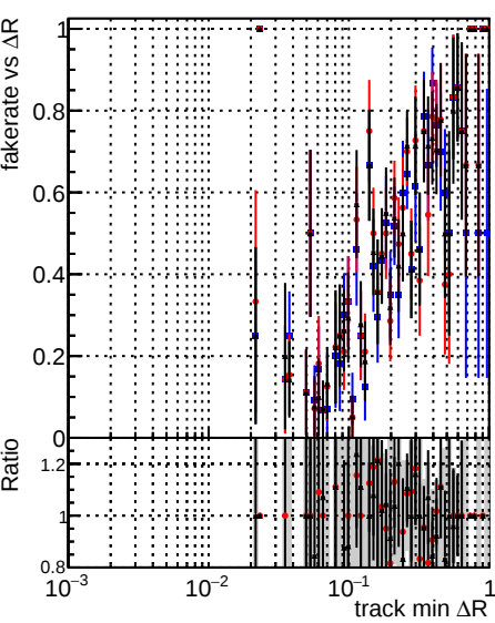
Fake rate vs ΔR(track, jet) DQM_original_step2_ttbar-phase1-newgeom DQM_pixelCPETemplate_step2_ttbar-phase1-newgeom DQM_pixelCPETemplateCutChiSquareNew6_step2_ttbar-phase1-newgeom
