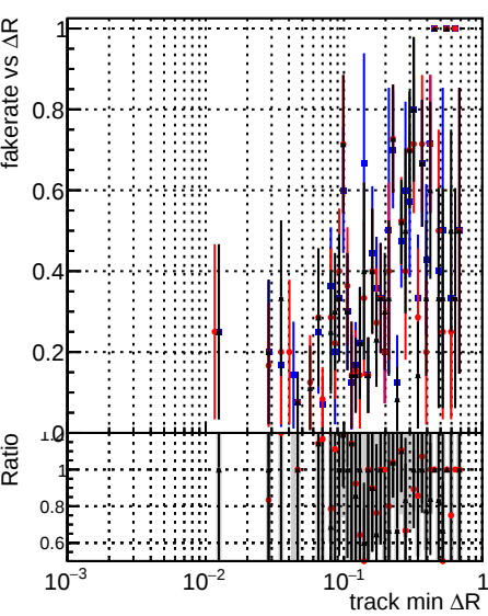
Fake rate vs \Delta R (track, jet) DQM_original_step2_ttbar-phase1-newgeom DQM_pixelCPETemplate_step2_ttbar-phase1-newgeom DQM_pixelCPETemplateCutChiSquareNew6_step2_ttbar-phase1-newgeom
