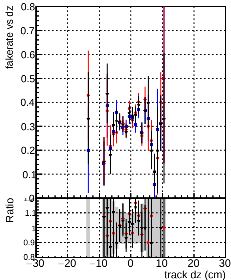
Fake rate vs dz — DOM original_step2_tbar-phase1-newgeom — DOM pixelCPE-template_step2_tbar-phase1-newgeom — DOM pixelCPE-template-cutchisquare-newgeom_step2_tbar-phase1-newgeom
