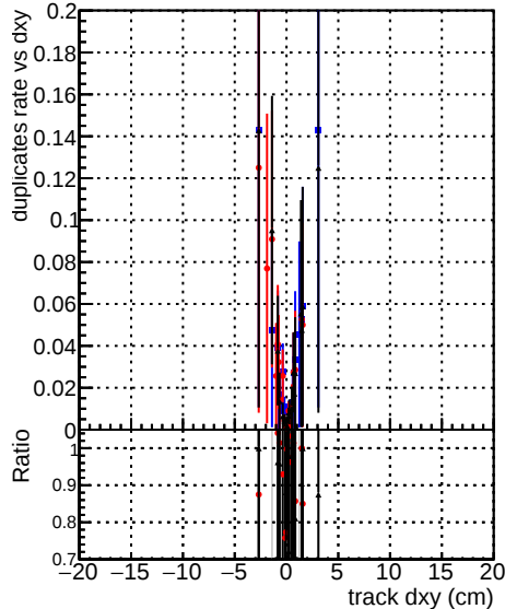
ttbar-phase1-newgeom SquareNew6 step2 ttbar-phase1-newgeom
