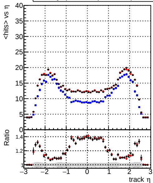
mean hits vs \eta Legend: DQM_original_step2_ttbar-phase1-newgeom (blue line) DQM_pixelCPETemplate_step2_ttbar-phase1-newgeom (red line) DQM_pixelCPETemplateCutChiSquareNew6_step2_ttbar-phase1-newgeom (black line)
