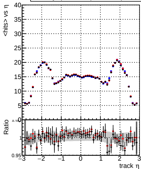
mean hit — DQM_original_step2_ttbar-phase1-newgeom — DQM_pixelCPETemplate_step2_ttbar-phase1-newgeom — DQM_pixelCPETemplateCutChiSquareNew6_step2_ttbar-phase1-newgeom
