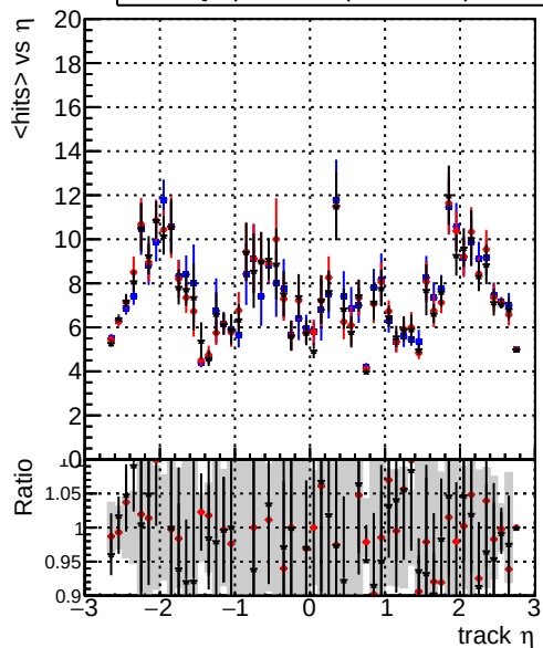
mean hit — DQM_original_step2_ttbar-phase1-newgeom — DQM_pixelCPETemplate_step2_ttbar-phase1-newgeom — DQM_pixelCPETemplateCutChiSquareNew6_step2_ttbar-phase1-newgeom
