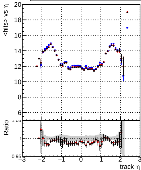
mean hits — DQM_original_step2_ttbar-phase1-newgeom — DQM_pixelCPETemplate_cut2_ttbar-phase1-newgeom — DQM_pixelCPETemplateCutChiSquareNew6_step2_ttbar-phase1-newgeom
