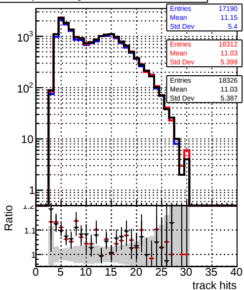
mean hits — DQM_original_step2_ttbar-phase1-newgeom — DQM_pixelCPETemplate_step2_ttbar-phase1-newgeom — DQM_pixelCPETemplateCutChiSquareNew6_step2_ttbar-phase1-newgeom
