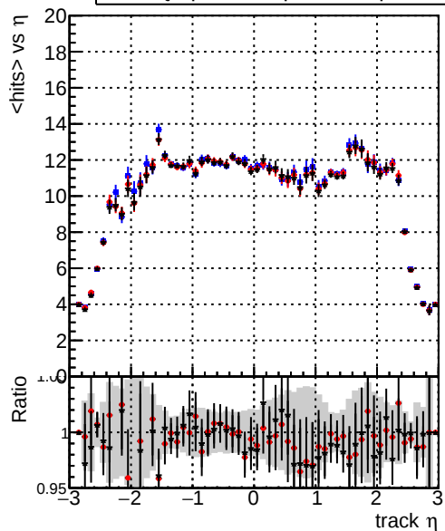
mean hits — DQM_original_step2_ttbar-phase1-newgeom — DQM_pixelCPETemplate_step2_ttbar-phase1-newgeom — DQM_pixelCPETemplateCutChiSquareNew6_step2_ttbar-phase1-newgeom
