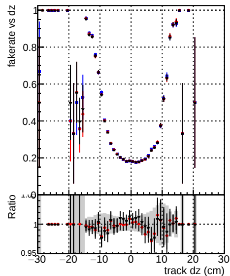
Fake rate vs dz Legend: DOM original_step2_tbar-phase1-newgeom DOM pixelCPE-template_step2_tbar-phase1-newgeom DOM pixelCPE-template-cutnewgeom
