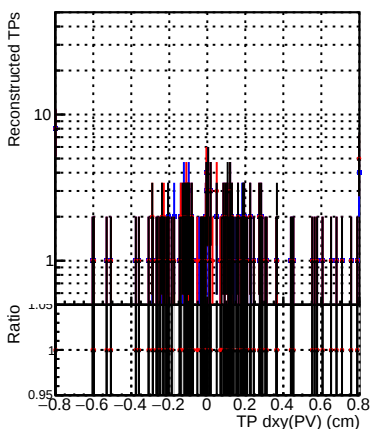
2_ttbar-phase1-newgeom
