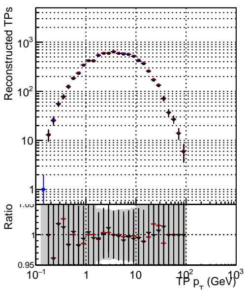
—•— DQM_original_step2_ttbbar-phase1-newgeom —•— DQM_pixelCPETemplate_step2_ttbbar-phase1-newgeom —•— DQM_pixelCPETemplateCutChiSquareNew6_step2_ttbbar-phase1-newgeom
