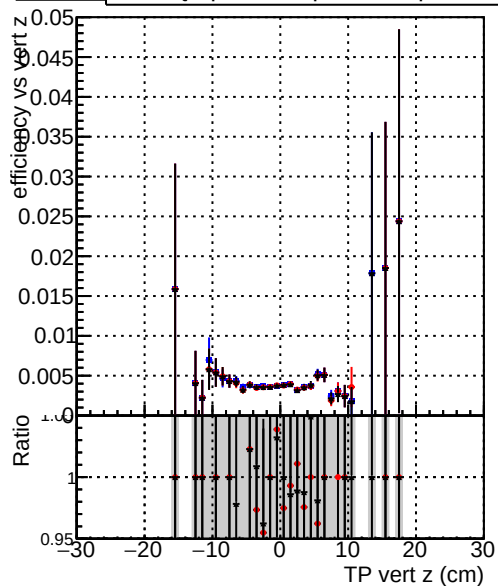
Efficiency vs TP vert z (cm) —•— DQM_original_step2_ttbar-phase1-newgeom —•— DQM_pixelCPETemplate_step2_ttbar-phase1-newgeom —•— DQM_pixelCPETemplateCutChiSquareNew6_step2_ttbar-phase1-newgeom
