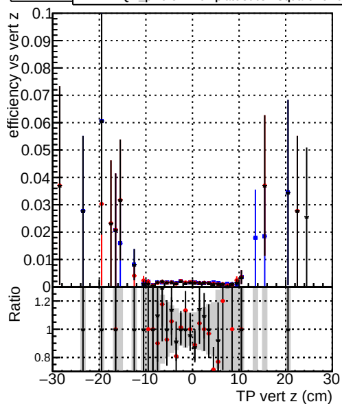
Efficiency vs. sim PV z — DQM_original_step2_ttbar-phase1-newgeom — DQM_pixelCPETemplate_step2_ttbar-phase1-newgeom — DQM_pixelCPETemplateCutChiSquareNew6_step2_ttbar-phase1-newgeom
