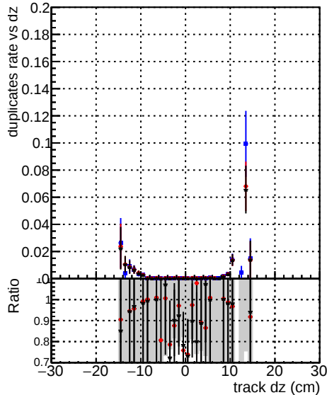
ttbar-phase1-newgeom SquareNew6_step2_ttbar-phase1-newgeom
