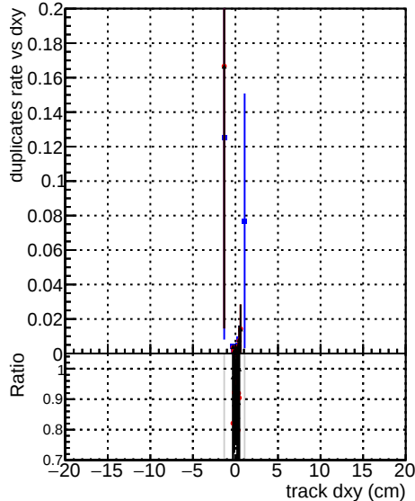
ttbar-phase1-newgeom SquareNew6_step2_ttbar-phase1-newgeom
