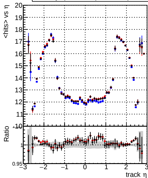
mean hits vs \eta — DQM_original_step2_ttbar-phase1-newgeom — DQM_pixelCPETemplate_step2_ttbar-phase1-newgeom — DQM_pixelCPETemplateCutChiSquareNew6_step2_ttbar-phase1-newgeom
