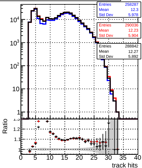
mean hits — DQM_original_step2_ttbar-phase1-newgeom — DQM_pixelCPETemplate_step2_ttbar-phase1-newgeom — DQM_pixelCPETemplateCutChiSquareNewv6_step2_ttbar-phase1-newgeom
