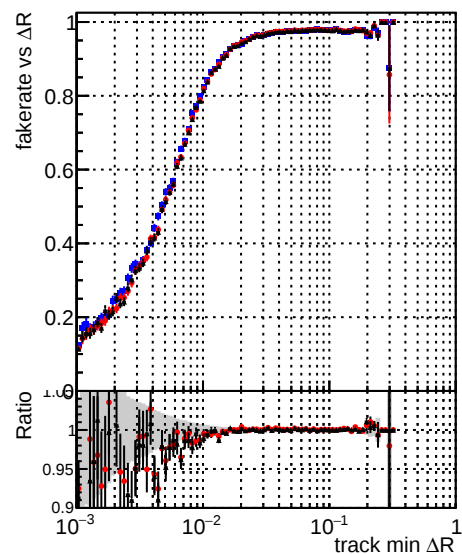
DQM_original_step2_ttbar-phase1-newgeom DQM_pixelCPETemplateCut2_ttbar-phase1-newgeom DQM_pixelCPETemplateCutChiSquareNew5_step2_ttbar-phase1-newgeom
