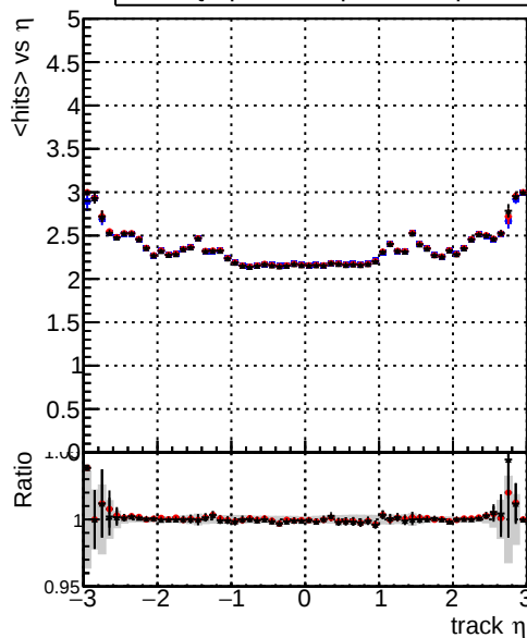
mean hits — DQM_original_step2_ttbar-phase1-newgeom — DQM_pixelCPETemplate_step2_ttbar-phase1-newgeom — DQM_pixelCPETemplateCutChiSquareNew5_step2_ttbar-phase1-newgeom
