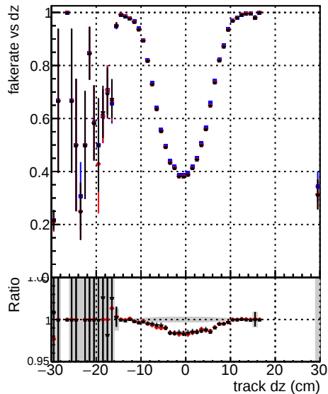
DOM original_step2_ttbare-phase1-newgeom pixelCPEtemplate_step2_ttbare-phase1-newgeom DOM_pixelCPEtemplate_cutsquarenew5_step2_ttbare-phase1-newgeom
