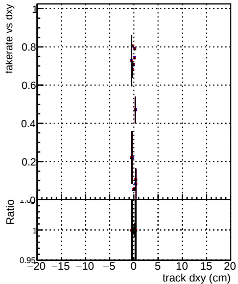
DOM original_step2_ttbarephase1-newgeom DOM pixelCPEtemplate_step2_ttbarephase1-newgeom DOM pixelCPEtemplatecutchisquarenew5_step2_ttbarephase1-newgeom
