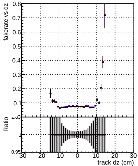
DOM original_step2_ttbarephase1-newgeom DOM pixelCPEtemplate_step2_ttbarephase1-newgeom DOM pixelCPEtemplatecutchisquarenew5_step2_ttbarephase1-newgeom
