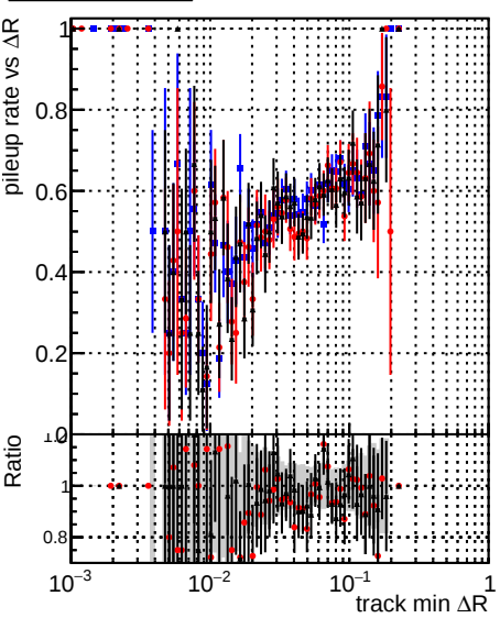
Legend: DQM_original_step2_ttbar-phase1-newgeom (blue), DQM_pixelCPETemplate_step2_ttbar-phase1-newgeom (red), DQM_pixelCPETemplateCutChiSquareNew5_step2_ttbar-phase1-newgeom (black)
