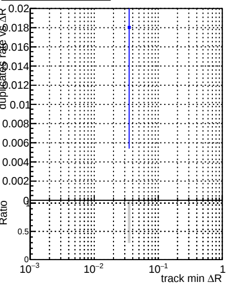
Legend: DQM_original_step2_ttbar-phase1-newgeom (blue), DQM_pixelCPETemplate_step2_ttbar-phase1-newgeom (red), DQM_pixelCPETemplateCutChiSquareNew5_step2_ttbar-phase1-newgeom (black)
