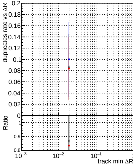
—●— DQM_original_step2_ttbar-phase1-newgeom —●— DQM_pixelCPETemplate_step2_ttbar-phase1-newgeom —●— DQM_pixelCPETemplateCutChiSquareNew5_step2_ttbar-phase1-newgeom
