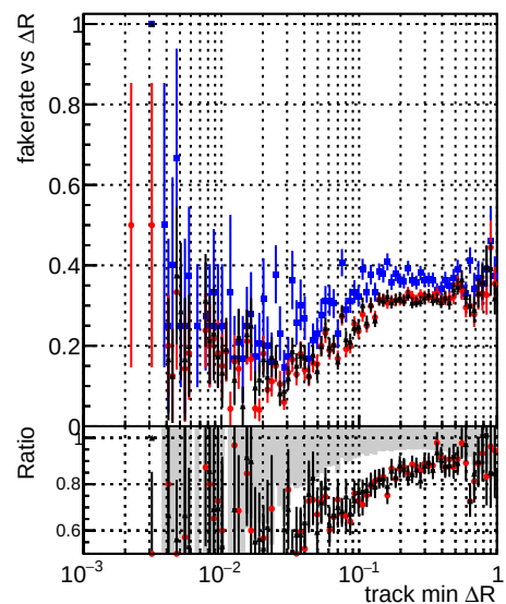
—●— DQM original step2 ttbar-phase1-newgeom —●— DQM pixelCPETemplate step2 ttbar-phase1-newgeom —●— DQM pixelCPETemplateCutChiSquareNew5_step2 ttbar-phase1-newgeom
