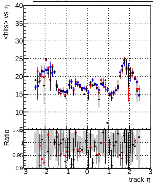
mean hit — DQM_original_step2_ttbbar-phase1-newgeom — DQM_pixelCPETemplate_step2_ttbbar-phase1-newgeom — DQM_pixelCPETemplateCutChiSquareNew5_step2_ttbbar-phase1-newgeom
