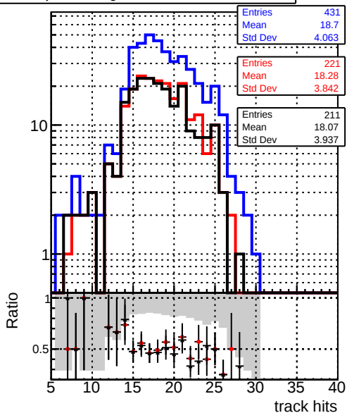
mean hit — DQM_original_step2_ttbbar-phase1-newgeom — DQM_pixelCPETemplate_step2_ttbbar-phase1-newgeom — DQM_pixelCPETemplateCutChiSquareNew5_step2_ttbbar-phase1-newgeom
